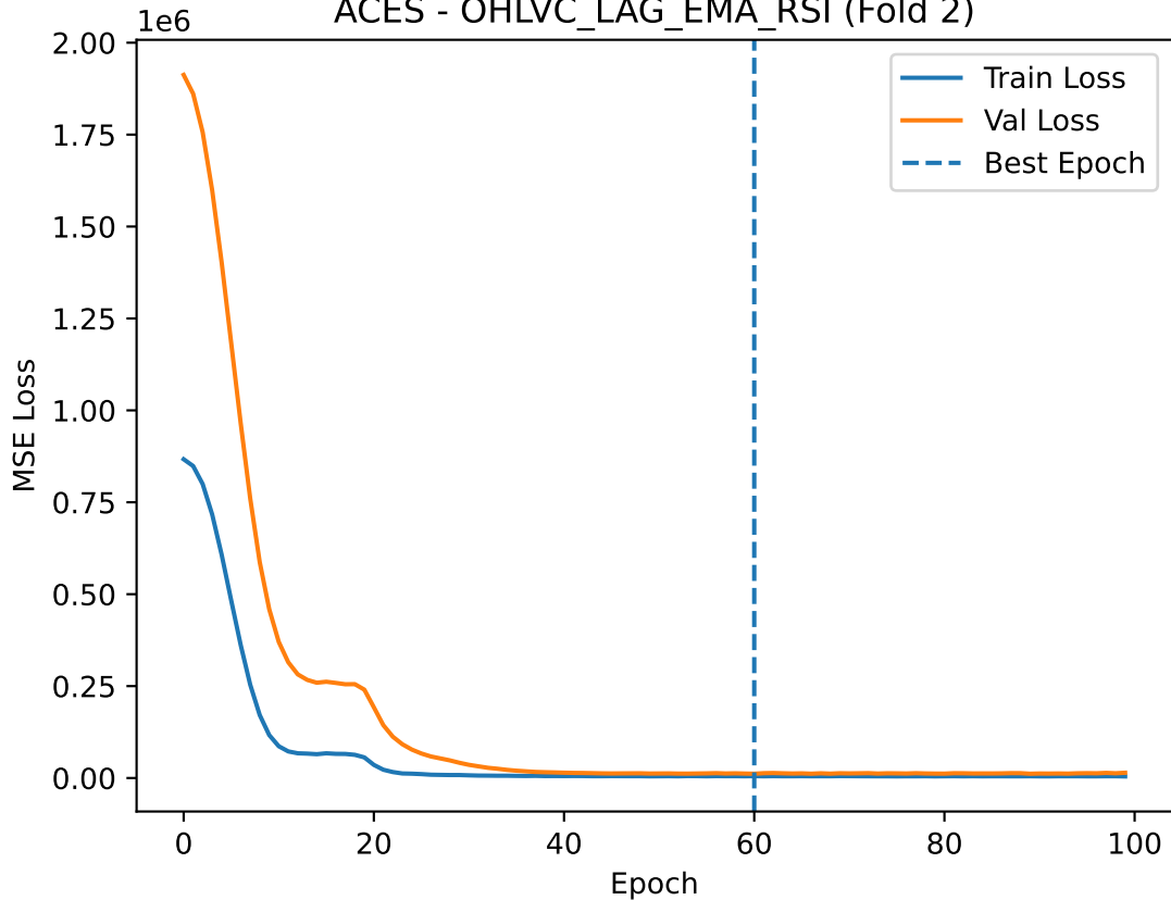
ACES - OHLVC_LAG_EMA_RSI (Fold 2)
